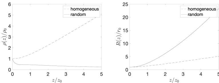
Figure 2. The correlation radius \rho(z) (left) and beam radius R(z) (right) when the source is such that \rho_o = 10\lambda_o , r_o = 100\lambda_o (with \lambda_o the wavelength), A_1 = A_2 = A_0 , and \chi = 0 as in Figure 1. We compare the functions in the homogeneous medium and in the random medium with scattering strength \bar{\gamma}_2 = 5 \cdot 10^{-7} \lambda_o^{-1} . Here z_o = k_o r_o \rho_o is the Rayleigh length of the partially coherent source and \bar{\gamma}_2 is defined by Eq. (30).
