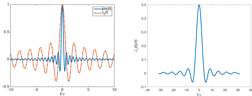
Figure 2. Left plot: the sinc function \text{sinc}(t) (solid line) and the Bessel function J_0(t) (dashed line) for t \in [-10\pi, 10\pi] . Right plot: the function \frac{J_1(|t|)}{|t|} for t \in [-10\pi, 10\pi] . The argument t is scaled by \pi in the abscissa.
