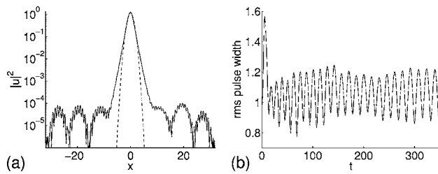
FIG. 3. Dynamics of a Gaussian pulse with initial mass N=1.02N_c=2.92 and radius a_0=a_c=1.4 ( a_{rms,0}=0.99 ). (a) The pulse profile at time t=350 (solid line) compared to the input Gaussian profile (dashed lines). (b) The rms pulse width vs time.
