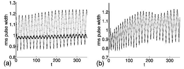
FIG. 2. Rms pulse width. (a) N=1.04N_c , a_0=0.63 ( a_{rms,0}=0.99 , solid line), a_0=0.75 ( a_{rms,0}=1.18 , dashed lines). (b) N=1.08N_c , a_0=0.5 ( a_{rms,0}=0.79 , solid line).
